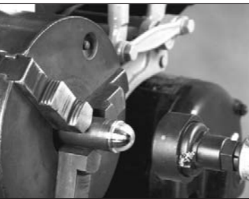
Lathe with Large Extended Series.
